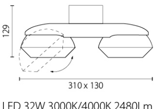
LED 32W 3000K/4000K 2480Lm
