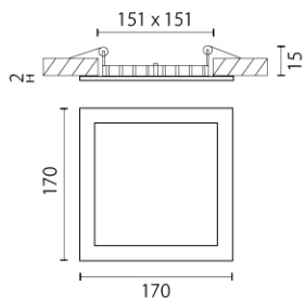
LED 12W 4000K 720Lm
