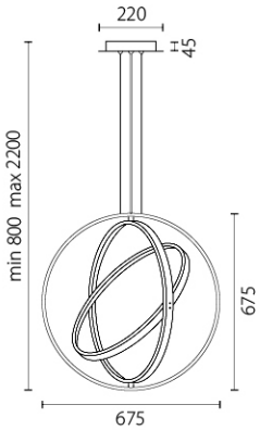
747122 LED 110W 3000K 9900Lm 747144 LED 110W 4000K 11000Lm
