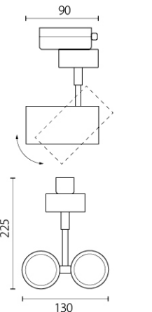
2 x Gu10 max 50W
