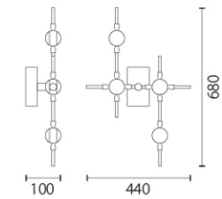
LED 20W 4000K 1600Lm
