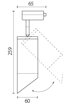
1 x Gu10 max 50W
