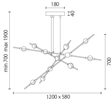
LED 60W 4000K 4800Lm
