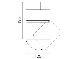
LED 26W 3000K/4000K 1950Lm
