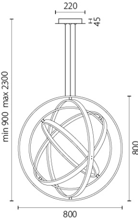
747222 LED 180W 3000K 16300Lm 747244 LED 180W 4000K 18000Lm
