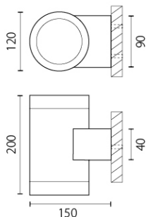
2 x DR111 LED 20W
