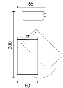
1 x Gu10 max 50W
