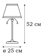
■ L17831.03 1 x E27 (60W)
