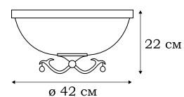
■ L17853.03 3 x E27 (60W)
