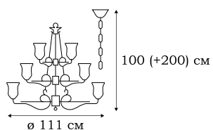
■ L17700.19 21 x E27 (60W)
