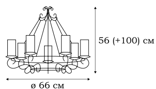
■ L18207.10 7 x E14 (60W)
