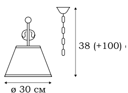
■ L17811.03 1 x E27 (60W)
