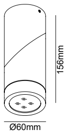
CLT 030C WH CODE:1400/102 Ø60xH156mm 1x35W MR16 GU10 IP54 CE
